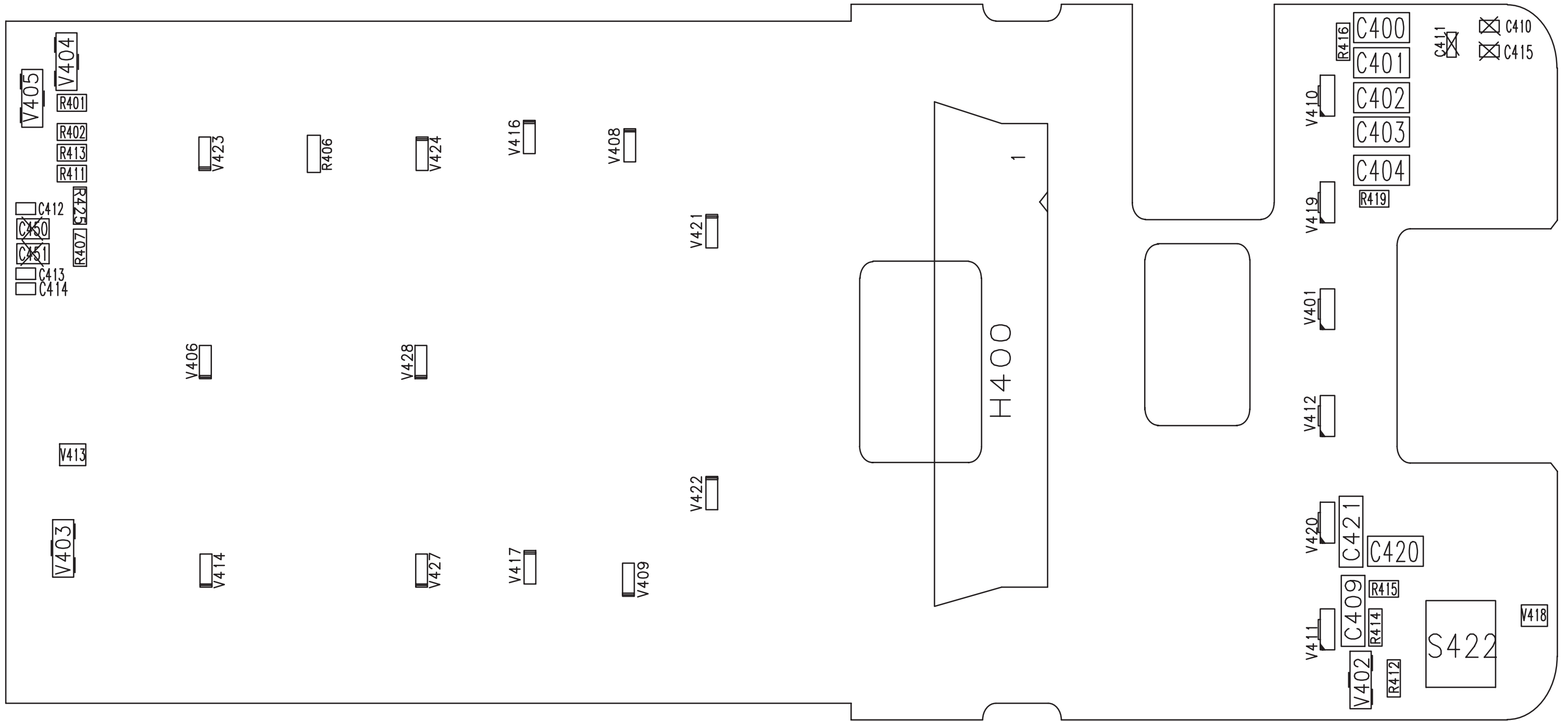
Figure 7 UIF Component Layout
